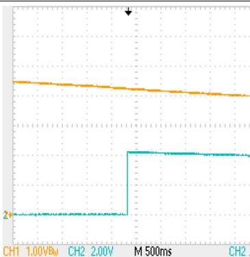
Figure 30. Initial Power Up, COUT
